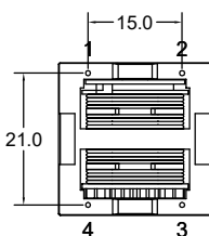
Bottom view
